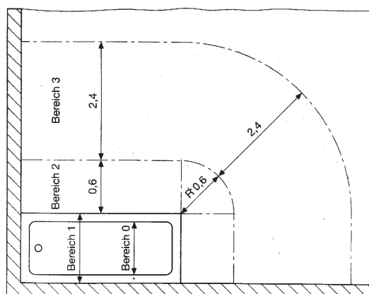
Example of classification of the area in rooms with bath.
